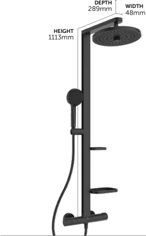
Round Two Function Shower System
