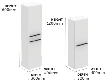
Column Unit - High, 2 doors
