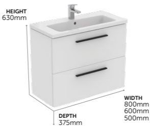
Compact Basin Unit, 2 Drawers
