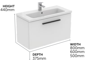
Compact Basin Unit, 1 Drawer
