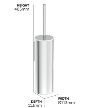
Toilet Brush & Holder N1396AA £118
