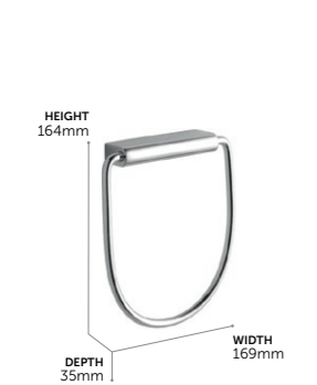
Towel Ring N1384AA £79
